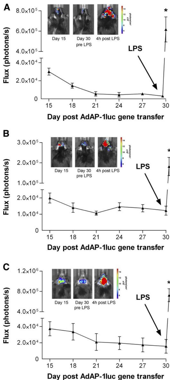
Fig. 4. Activator protein (AP)-1-driven luciferase expression is stable and inducible 1 mo after adenovirus-mediated gene transfer to central cardiovascular regulatory nuclei. Bioluminescence profiles following targeted AdAP-1luc delivery to the SFO (A, n = 4 ), PVN (B, n = 4 ), or RVLM (C, n = 7 ). Peak luminescence signal was monitored at every 2–4 days for 1 mo. At 30 days postgene transfer, systemic LPS challenge (8 \mu g/g ip) induced a robust increase in AP-1-dependent luminescence in all 3 nuclei. Inset images : typical bioluminescence overlays at defined time points. Areas of high photon emission are displayed as red, and areas of low photon emission are displayed as blue. * P < 0.05 vs. pre-LPS.
