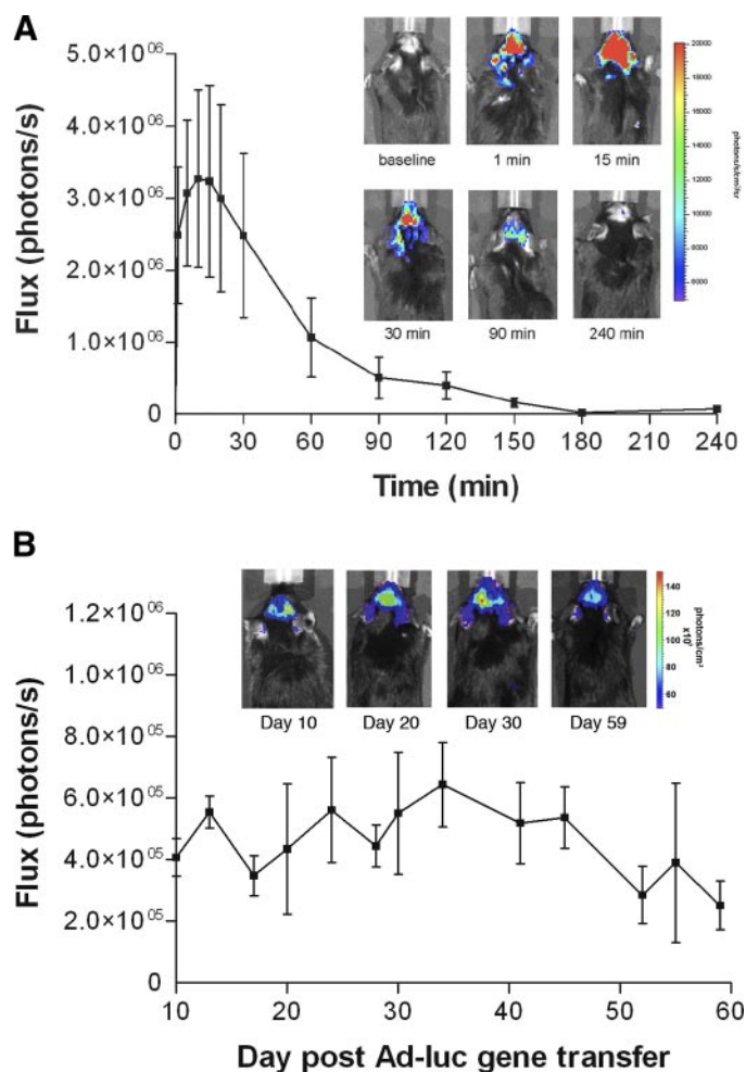
Fig. 1. Kinetics and long-term stability of the bioluminescence signal following adenovirus-mediated gene transfer of cytomegalovirus (CMV)-driven luciferase to the subformal organ (SFO). A: time-dependent decay of bioluminescence signal following luciferin administration (150 mg/kg ip) in mice 7 days following SFO-targeted gene transfer of AdCMVluc ( n = 4 ). Detectable luminescence (flux; photons/s) peaked 10–15 min following luciferin injection and decayed 90% by 4 h. Inset images: representative bioluminescence overlays prior to (baseline) and at defined time points following luciferin injection. Areas of highest photon detection are shown in red, and lower levels of detection are shown in blue. B: AdCMVluc-mediated bioluminescence remains stable and detectable for up to 2 mo after targeted gene transfer to the SFO. Following SFO-targeted gene transfer of CMV-driven luciferase ( n = 5 ), luminescence was measured 10 min after luciferin administration (150 mg/kg ip) every 3–7 days over the course of 2 mo. Inset: representative pseudo-color bioluminescence overlays at defined time points postgene transfer.
