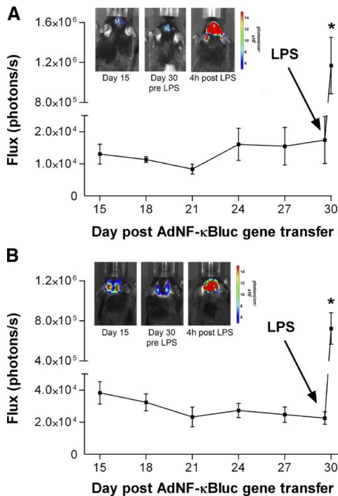
Fig. 3. NF- \kappa B-driven luciferase expression is stable and inducible 1 mo after gene transfer to the paraventricular nucleus (PVN) or rostral ventrolateral medulla (RVLM). Bioluminescence profiles following targeted AdNF- \kappa Bluc delivery to the PVN (A, n = 4 ) or RVLM (B, n = 6 ). Peak luminescence signal was monitored every 2–4 days for 1 mo. At 30 days postgene transfer, systemic LPS challenge (8 \mu g/g ip) induced a dramatic increase in NF- \kappa B-dependent luminescence in the PVN and RVLM. This dose of LPS was utilized to avoid increased mortality following higher (40 \mu g/g) doses of LPS observed in previous studies. Insets : typical bioluminescence overlays at defined time points. Areas of high photon emission are displayed as red, and areas of low photon emission are displayed as blue. * P < 0.05 vs. pre-LPS.
