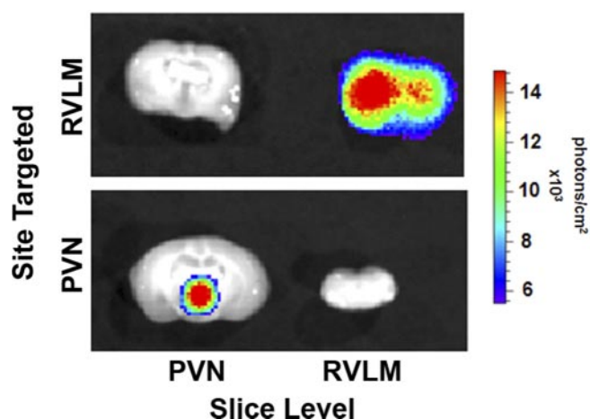
Fig. 5. AP-1-dependent luminescence is localized to brain regions targeted. One month following PVN or RVLN targeted delivery of AdAP-1luc, coronal brain sections (1 mm) were taken at the level of the PVN and RVLN 4 h following systemic LPS challenge (8 \mu\text{g/g} ip), and bioluminescence signal was visualized. Representative images of brain sections in which the AdAP-1-luc construct was targeted to the RVLN ( top ) or PVN ( bottom ) are shown. Areas of high photon emission are displayed as red, and areas of low photon emission are displayed as blue.
